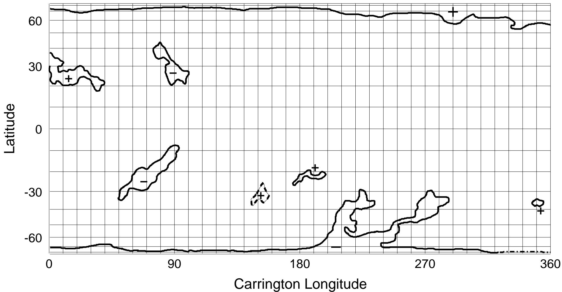
NSO/KP He I 1083 nm Coronal Hole Map: Carrington Rotation 1944
