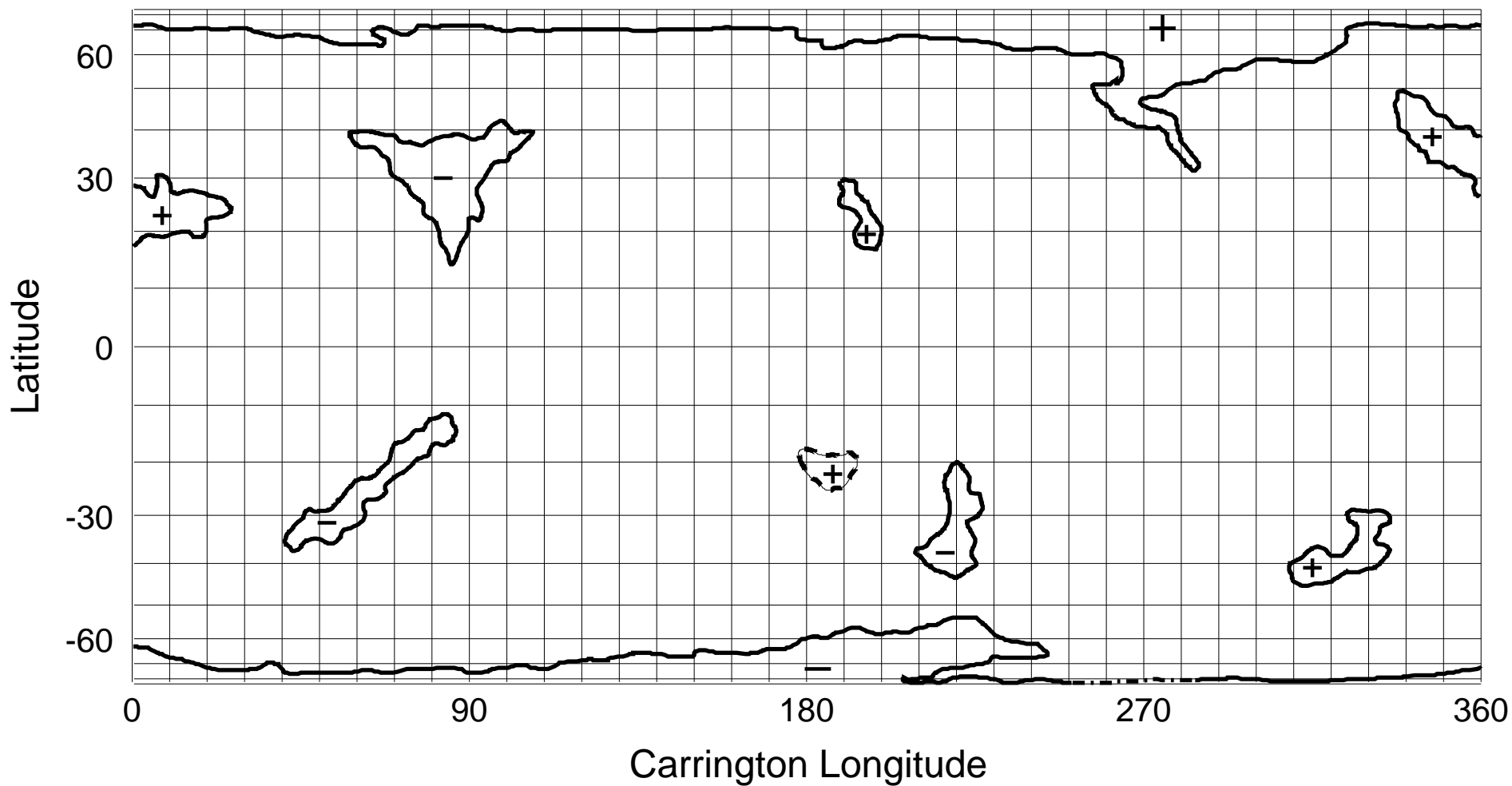
NSO/KP He I 1083 nm Coronal Hole Map: Carrington Rotation 1945
