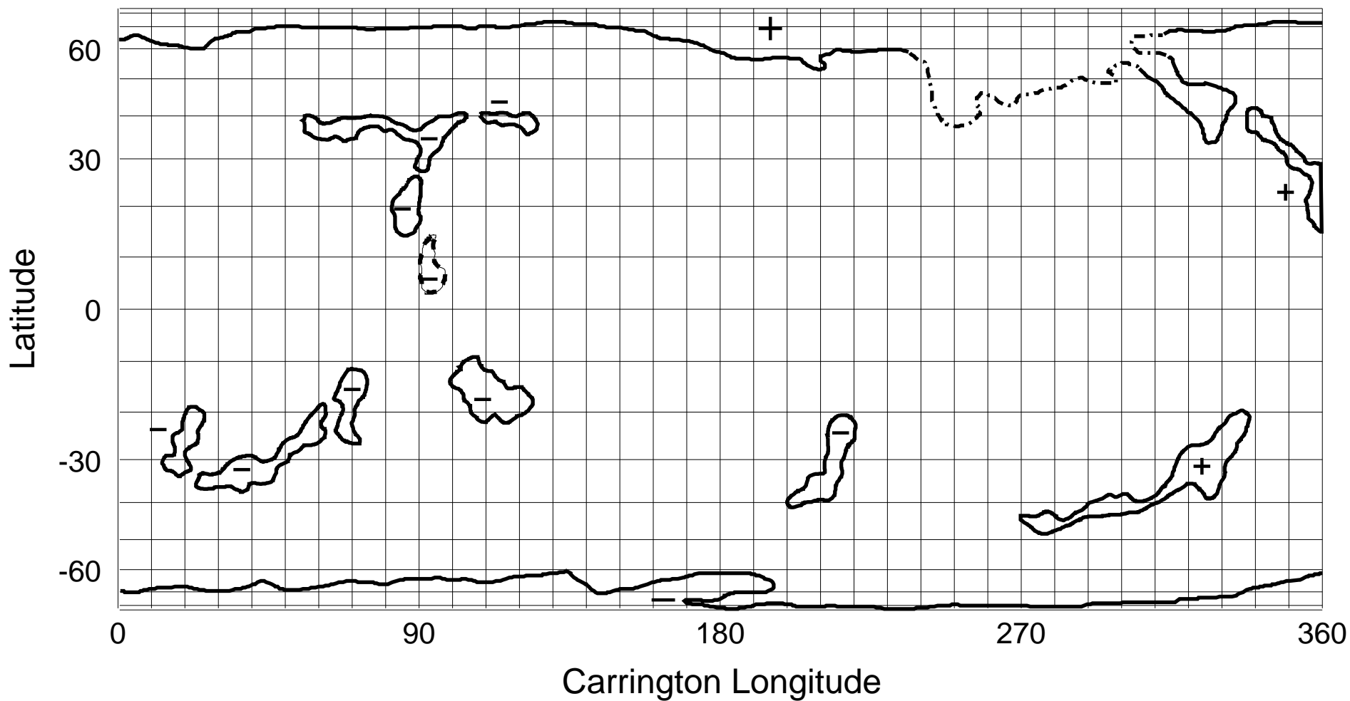
NSO/KP He I 1083 nm Coronal Hole Map: Carrington Rotation 1946
