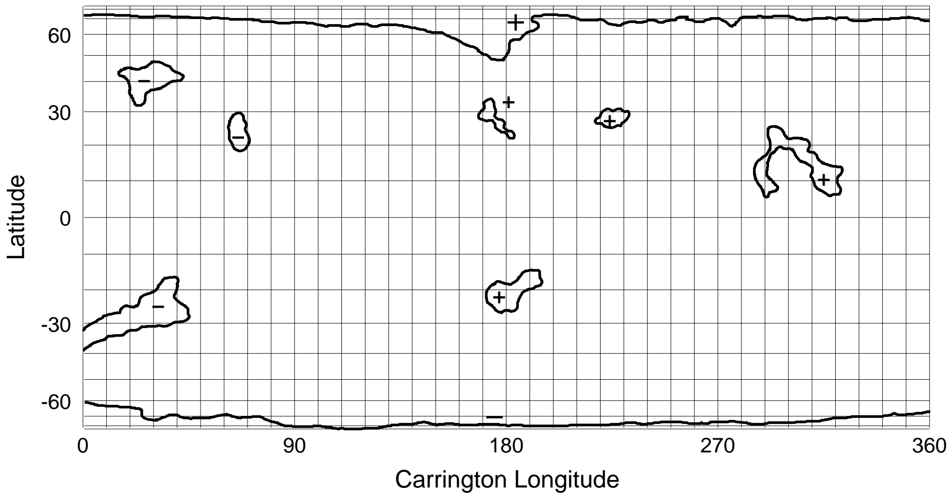
NSO/KP He I 1083 nm Coronal Hole Map: Carrington Rotation 1948
