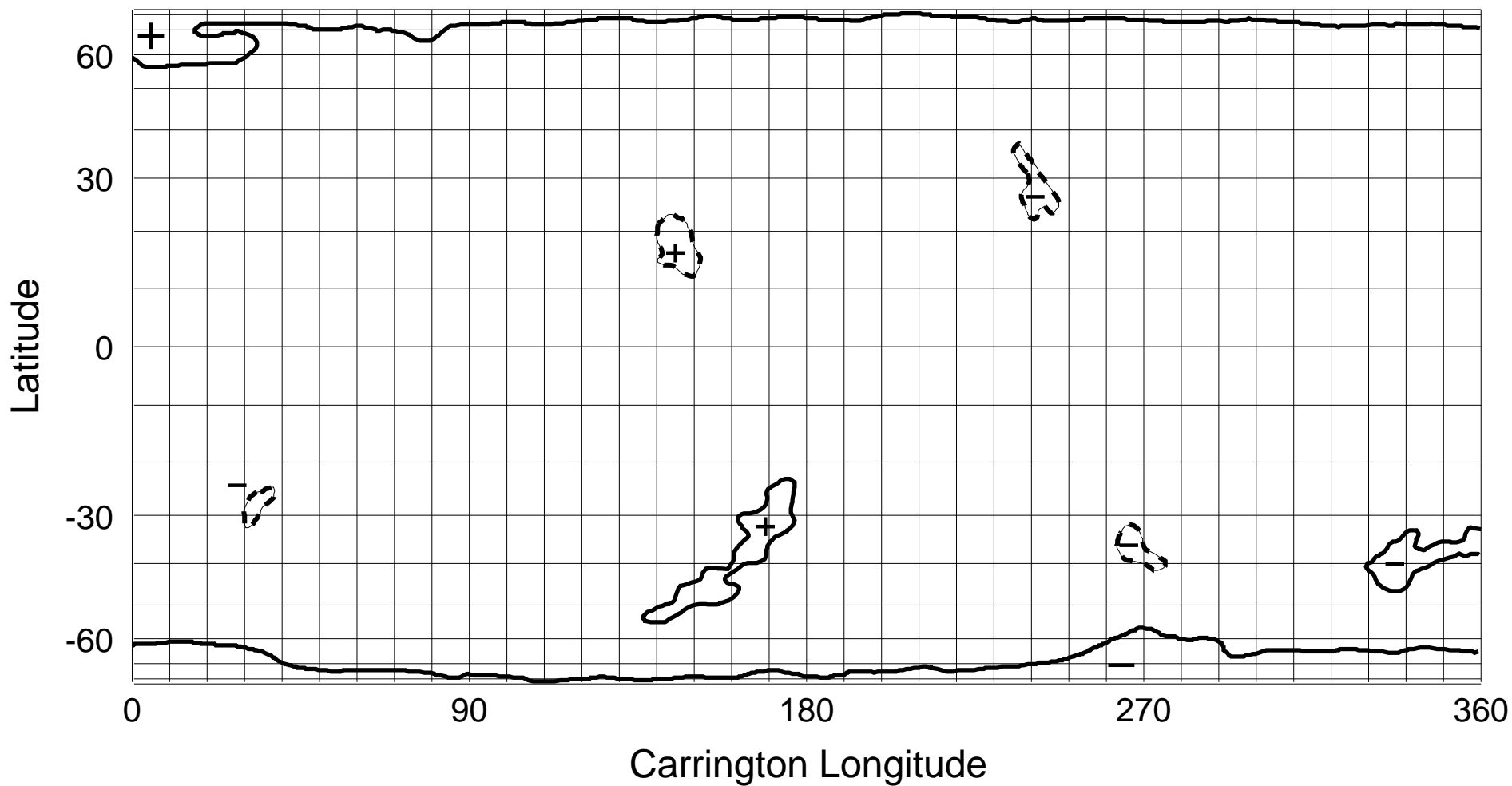
NSO/KP He I 1083 nm Coronal Hole Map: Carrington Rotation 1950
