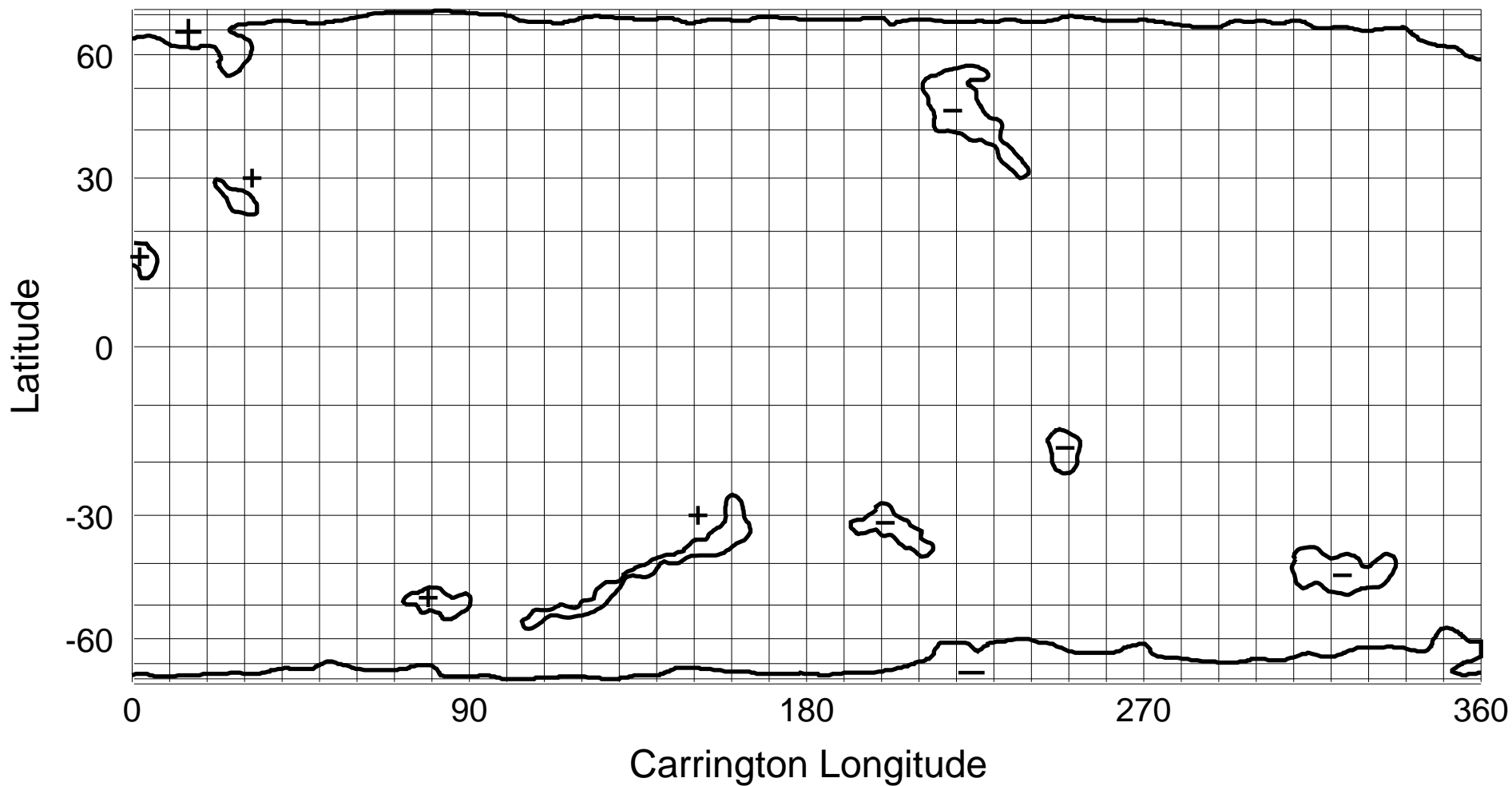
NSO/KP He I 1083 nm Coronal Hole Map: Carrington Rotation 1951
