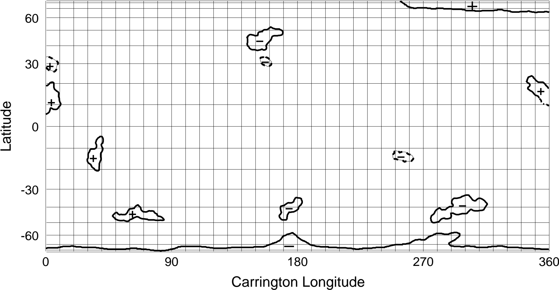
NSO/KP He I 1083 nm Coronal Hole Map: Carrington Rotation 1952
