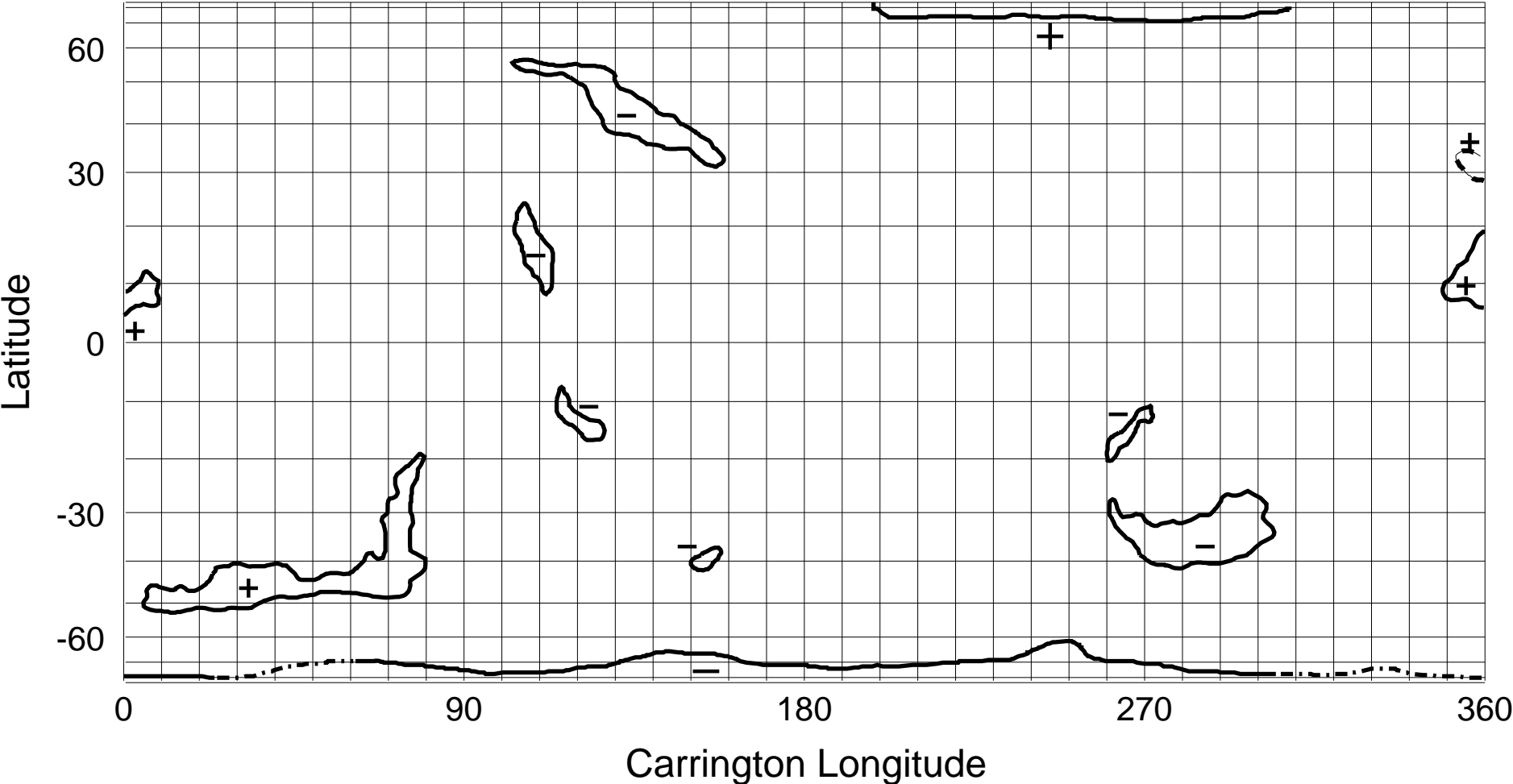
NSO/KP He I 1083 nm Coronal Hole Map: Carrington Rotation 1953
