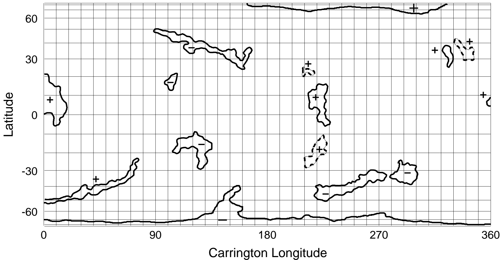
NSO/KP He I 1083 nm Coronal Hole Map: Carrington Rotation 1954
