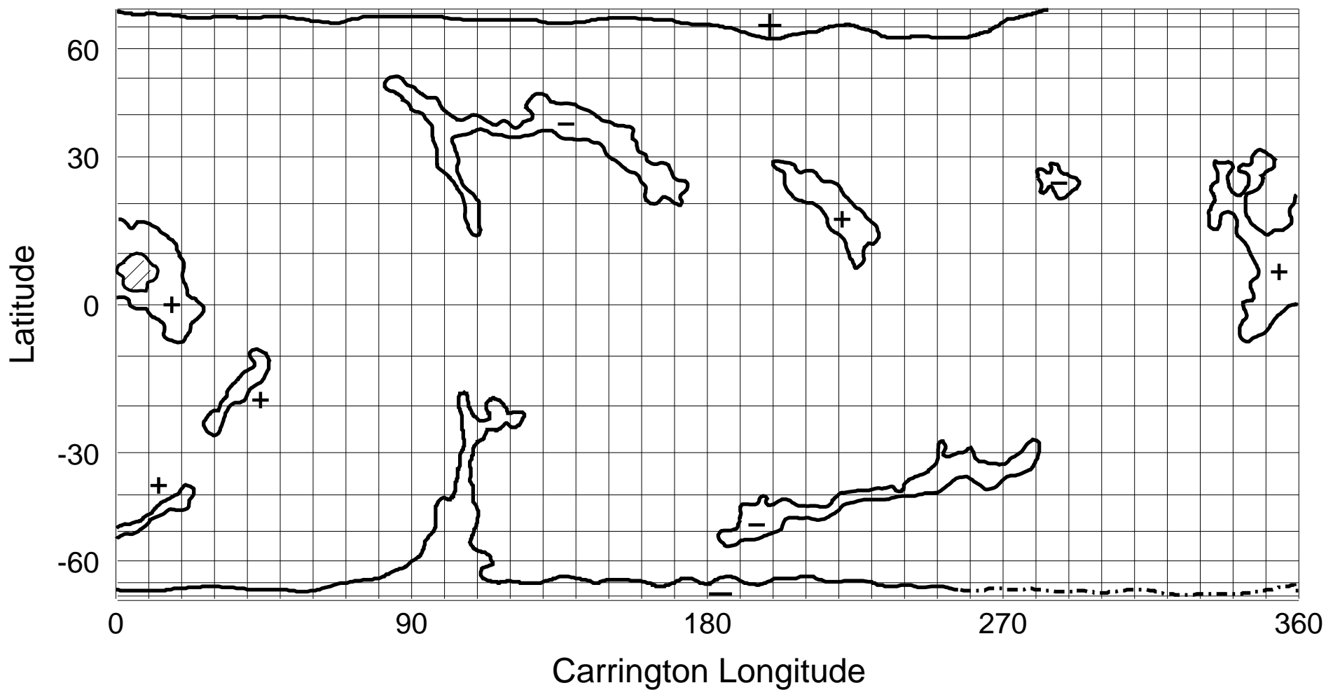
NSO/KP He I 1083 nm Coronal Hole Map: Carrington Rotation 1955
