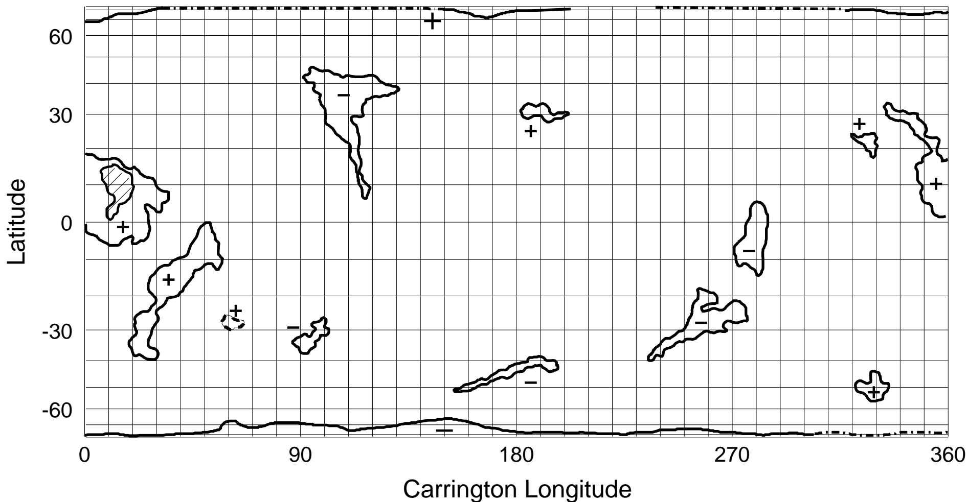
NSO/KP He I 1083 nm Coronal Hole Map: Carrington Rotation 1956
