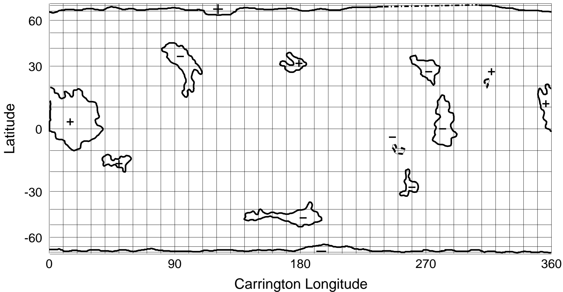
NSO/KP He I 1083 nm Coronal Hole Map: Carrington Rotation 1957
