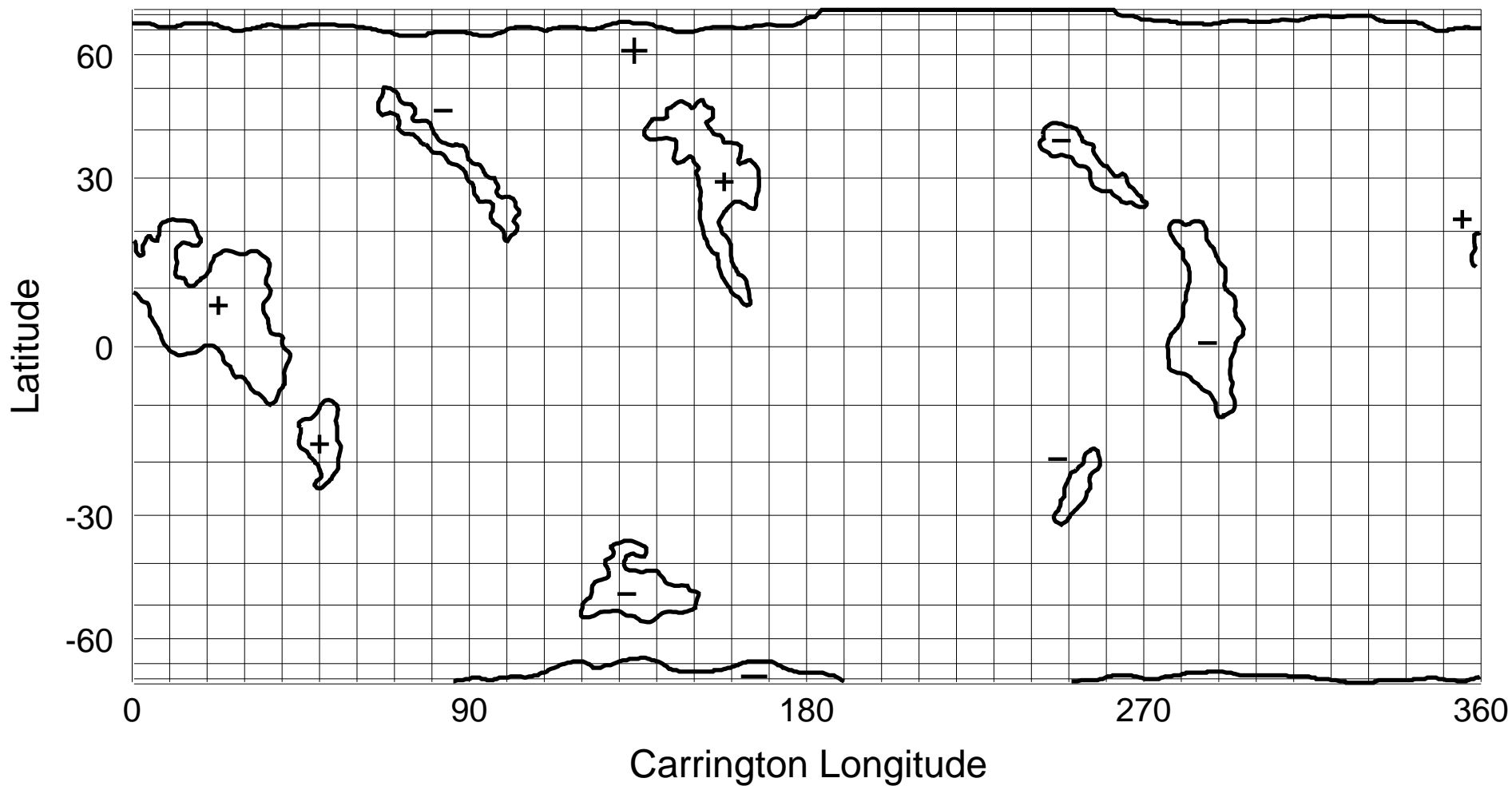
NSO/KP He I 1083 nm Coronal Hole Map: Carrington Rotation 1958
