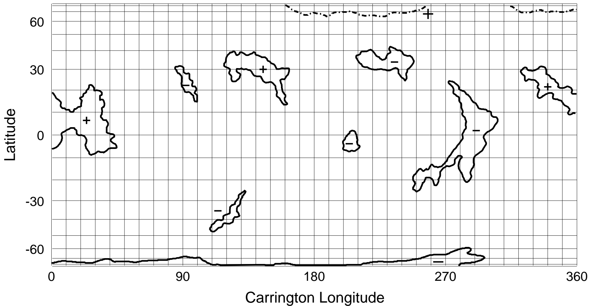
NSO/KP He I 1083 nm Coronal Hole Map: Carrington Rotation 1959
