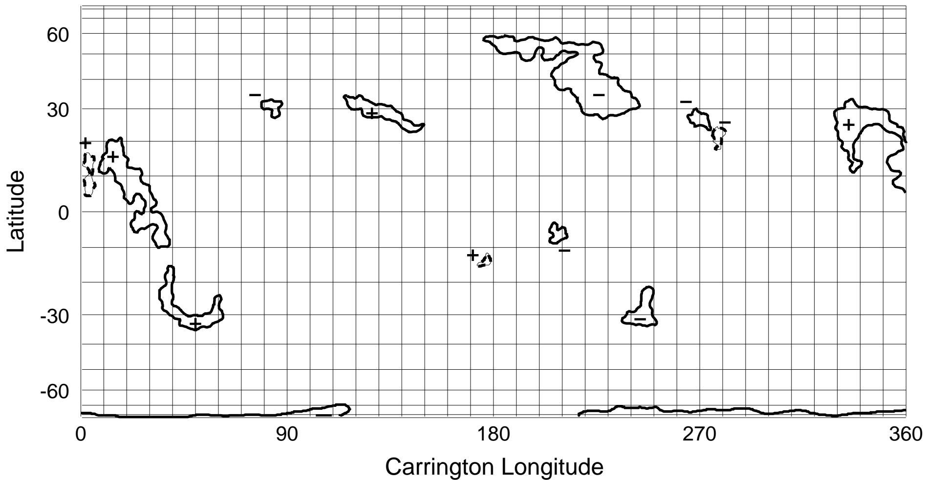
NSO/KP He I 1083 nm Coronal Hole Map: Carrington Rotation 1960
