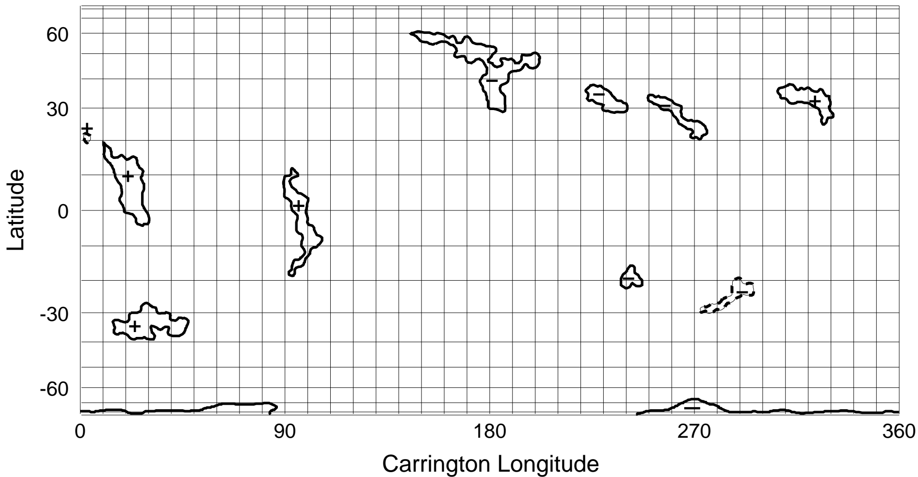
NSO/KP He I 1083 nm Coronal Hole Map: Carrington Rotation 1961
