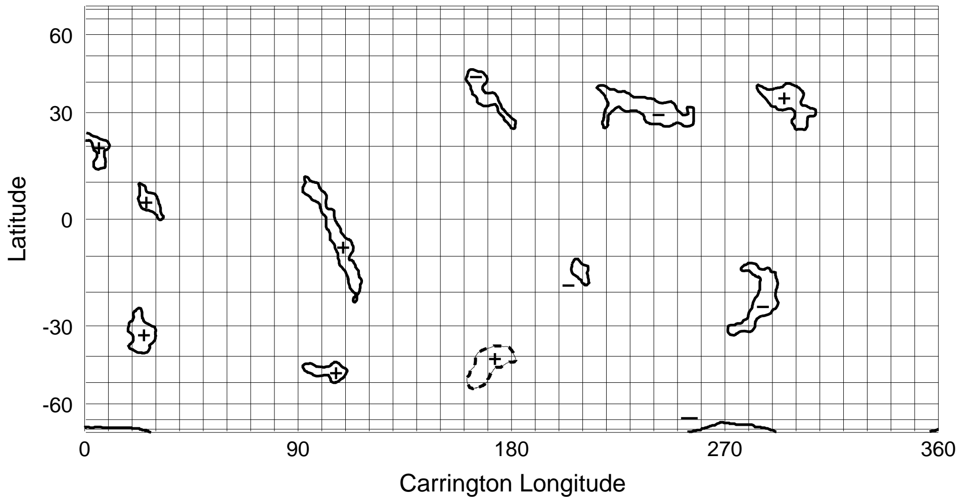
NSO/KP He I 1083 nm Coronal Hole Map: Carrington Rotation 1962
