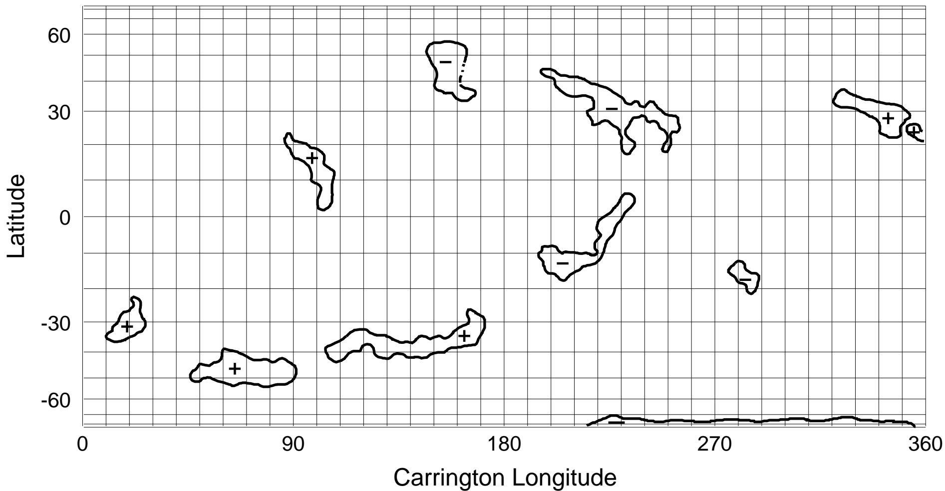
NSO/KP He I 1083 nm Coronal Hole Map: Carrington Rotation 1963
