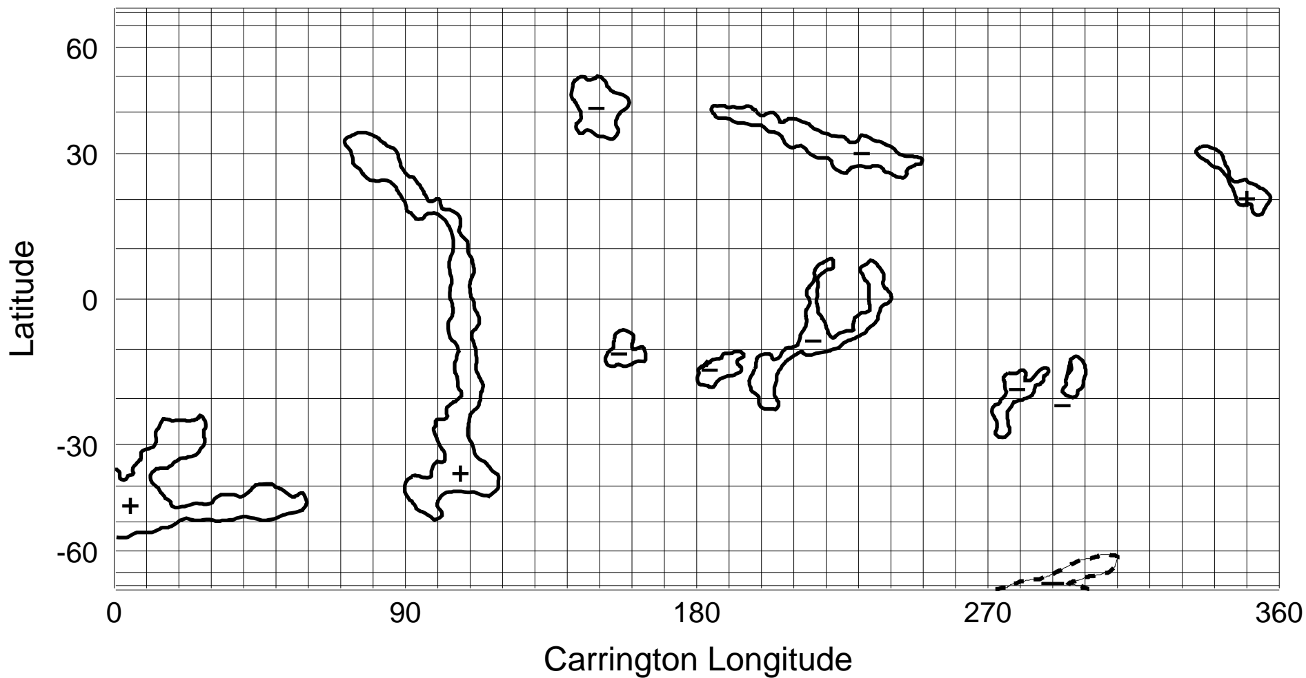
NSO/KP He I 1083 nm Coronal Hole Map: Carrington Rotation 1964
