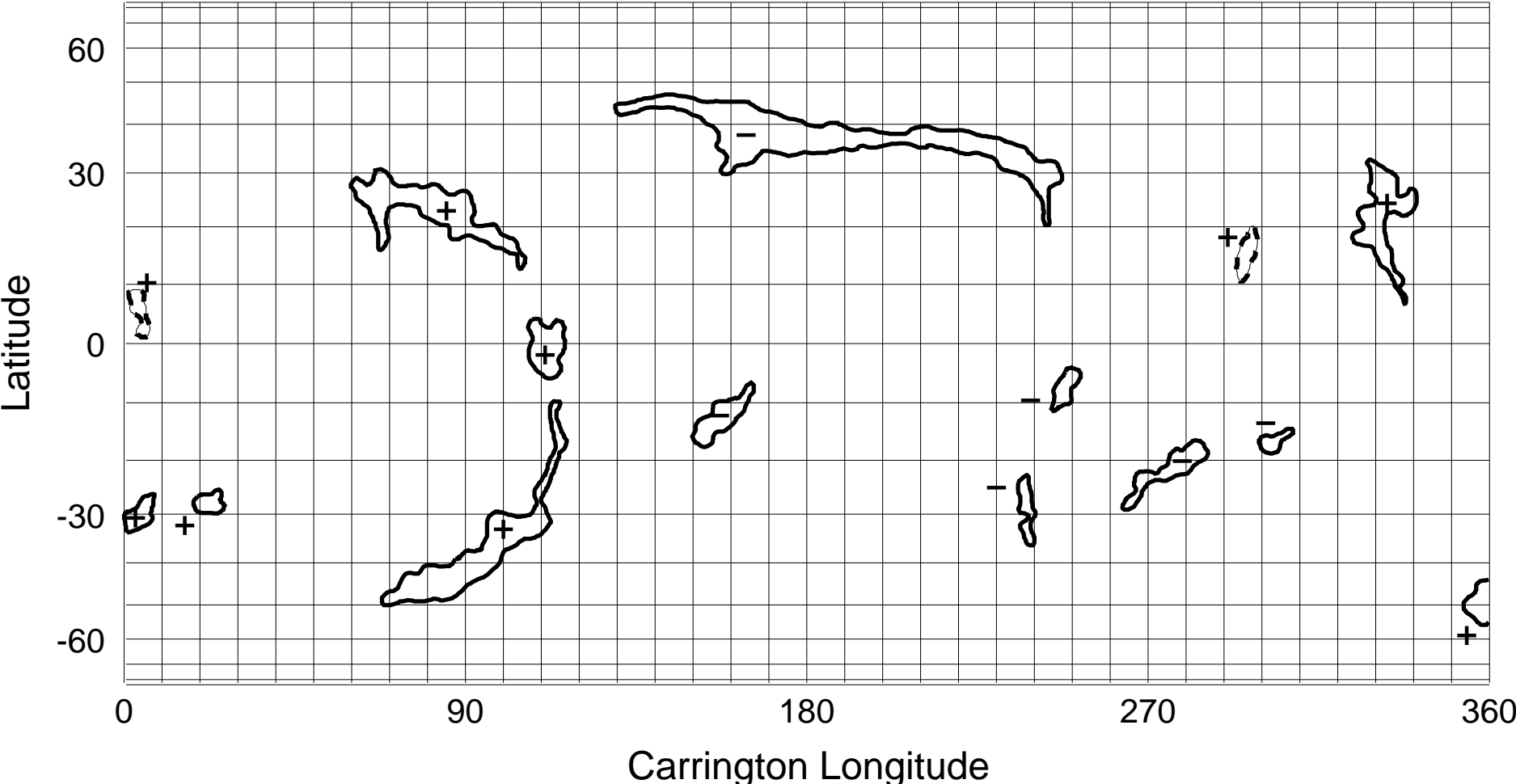
NSO/KP He I 1083 nm Coronal Hole Map: Carrington Rotation 1965
