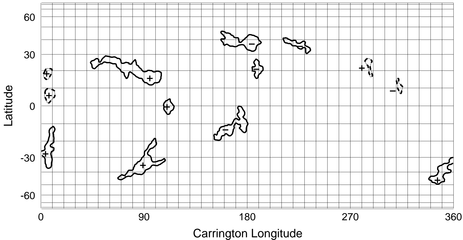
NSO/KP He I 1083 nm Coronal Hole Map: Carrington Rotation 1966
