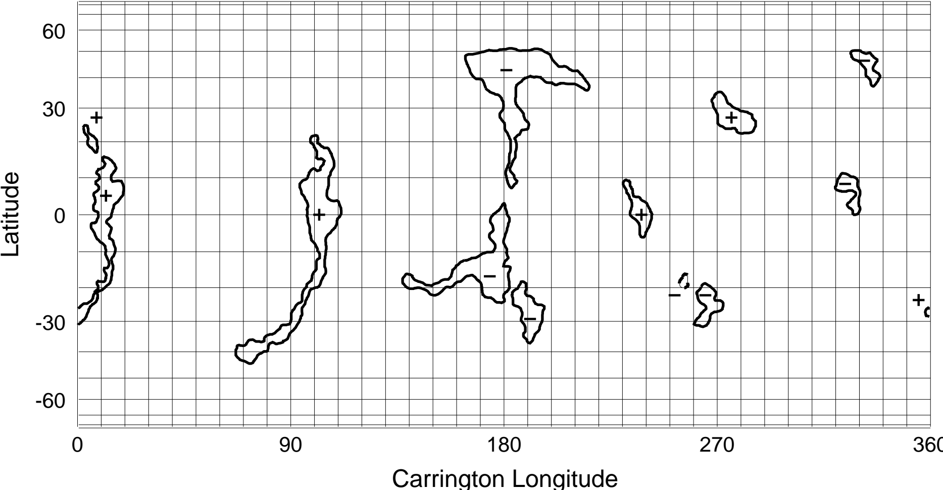
NSO/KP He I 1083 nm Coronal Hole Map: Carrington Rotation 1967
