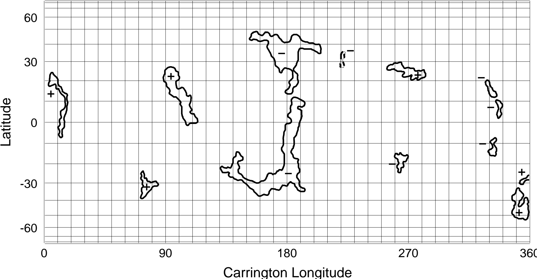
NSO/KP He I 1083 nm Coronal Hole Map: Carrington Rotation 1968
