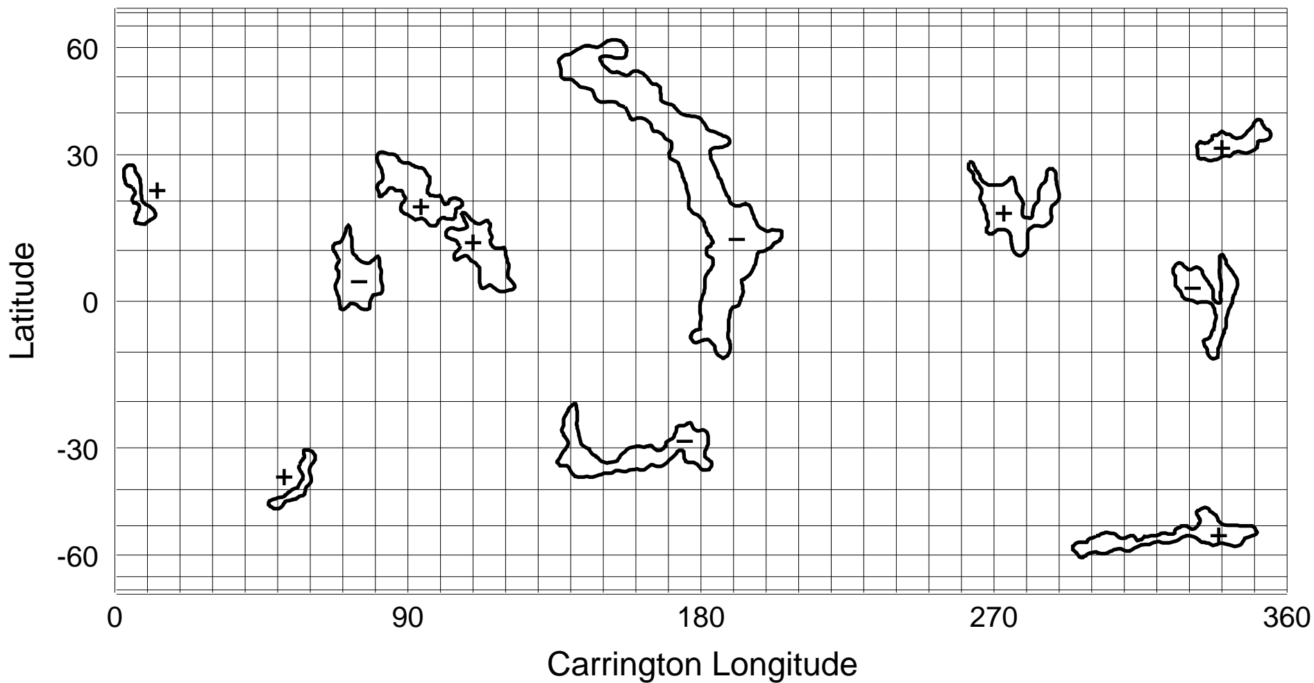
NSO/KP He I 1083 nm Coronal Hole Map: Carrington Rotation 1969
