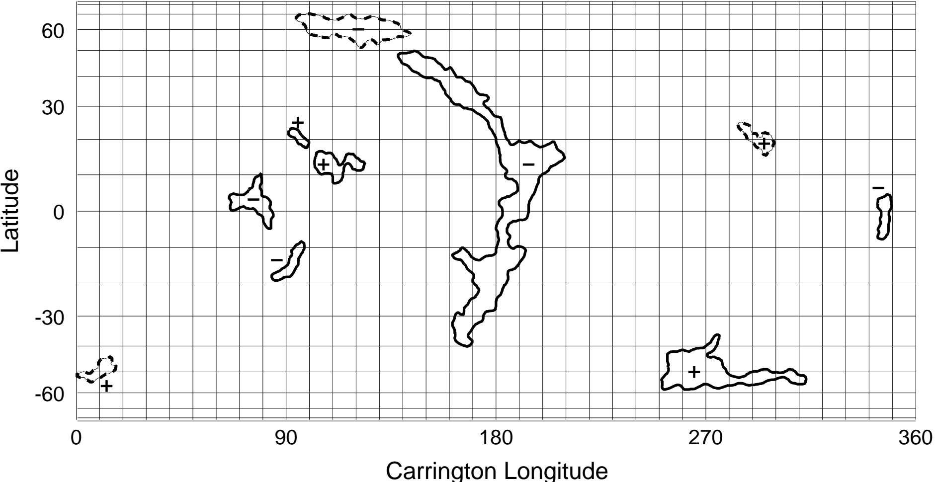
NSO/KP He I 1083 nm Coronal Hole Map: Carrington Rotation 1970
