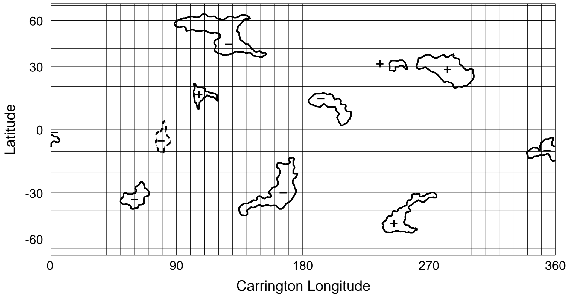
NSO/KP He I 1083 nm Coronal Hole Map: Carrington Rotation 1971
