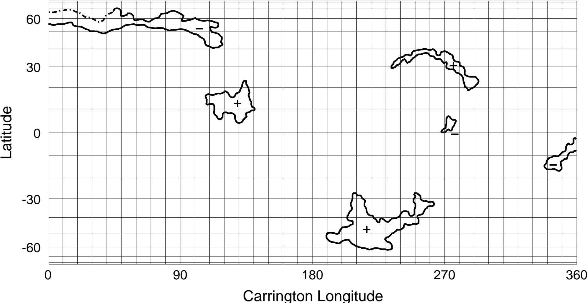
NSO/KP He I 1083 nm Coronal Hole Map: Carrington Rotation 1972
