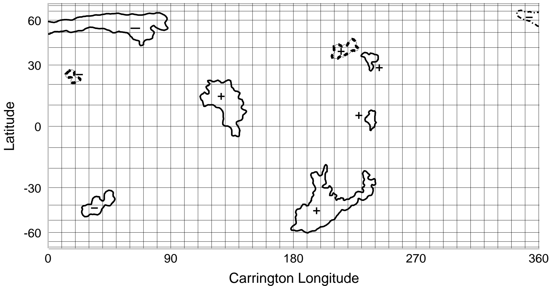
NSO/KP He I 1083 nm Coronal Hole Map: Carrington Rotation 1973
