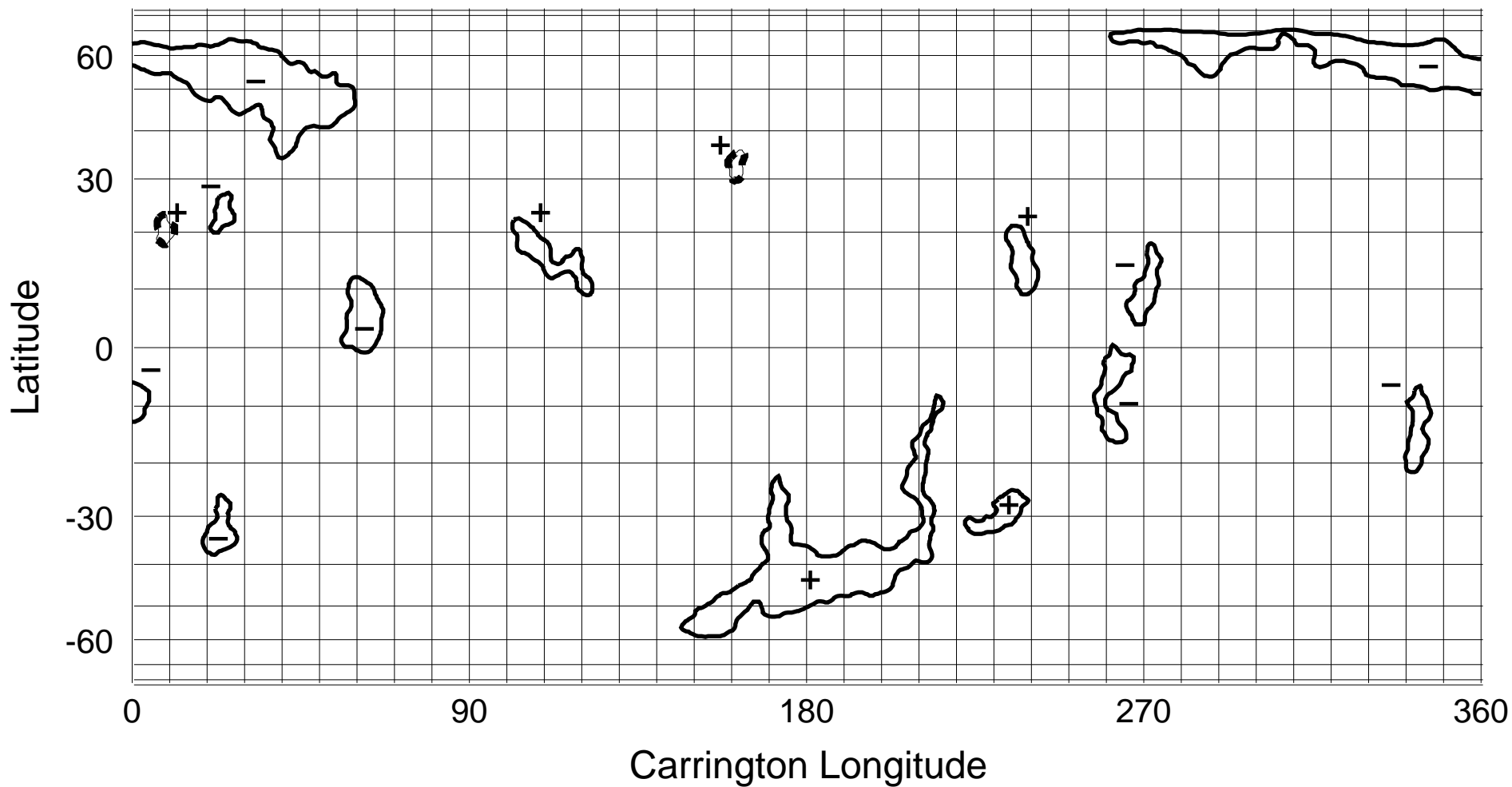
NSO/KP He I 1083 nm Coronal Hole Map: Carrington Rotation 1974
