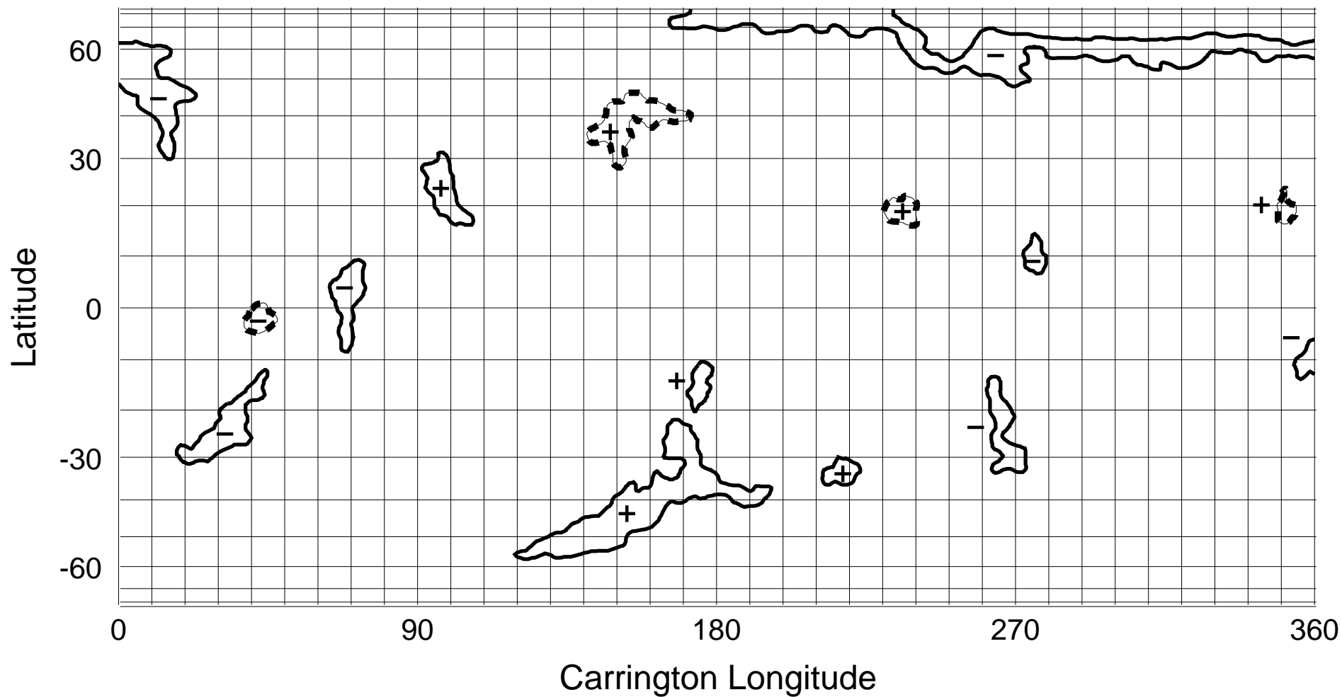
NSO/KP He I 1083 nm Coronal Hole Map: Carrington Rotation 1975
