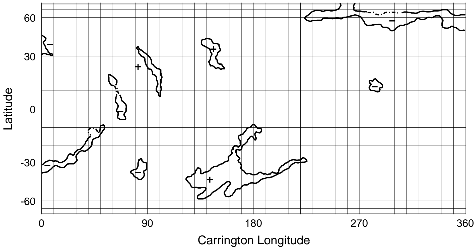
NSO/KP He I 1083 nm Coronal Hole Map: Carrington Rotation 1976
