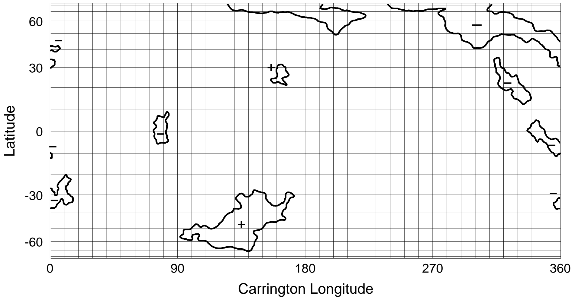
NSO/KP He I 1083 nm Coronal Hole Map: Carrington Rotation 1977
