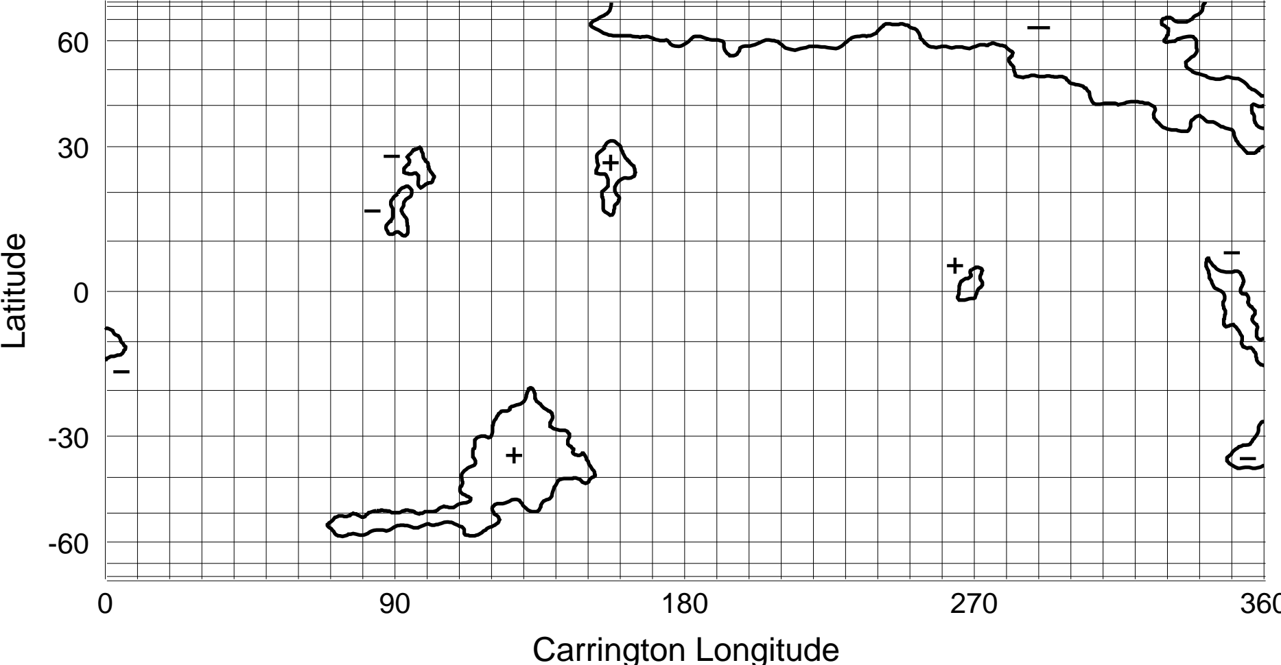
NSO/KP He I 1083 nm Coronal Hole Map: Carrington Rotation 1978
