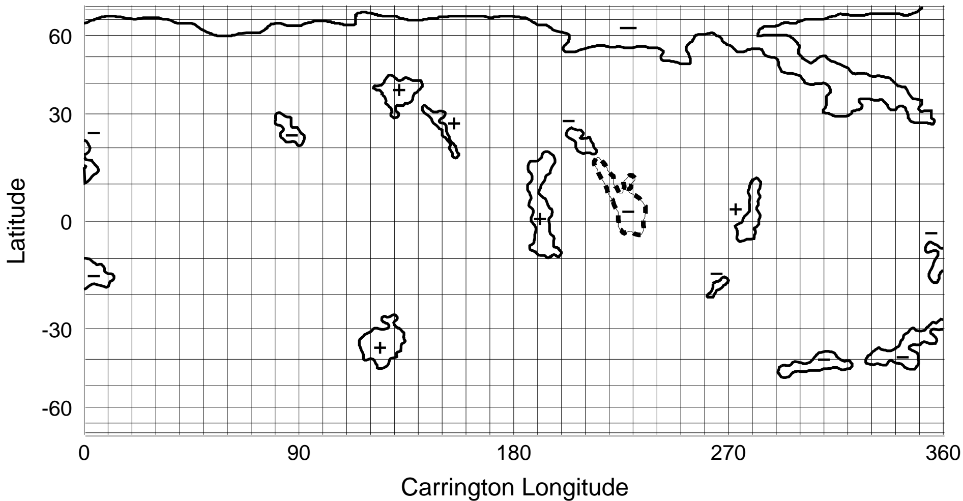
NSO/KP He I 1083 nm Coronal Hole Map: Carrington Rotation 1979
