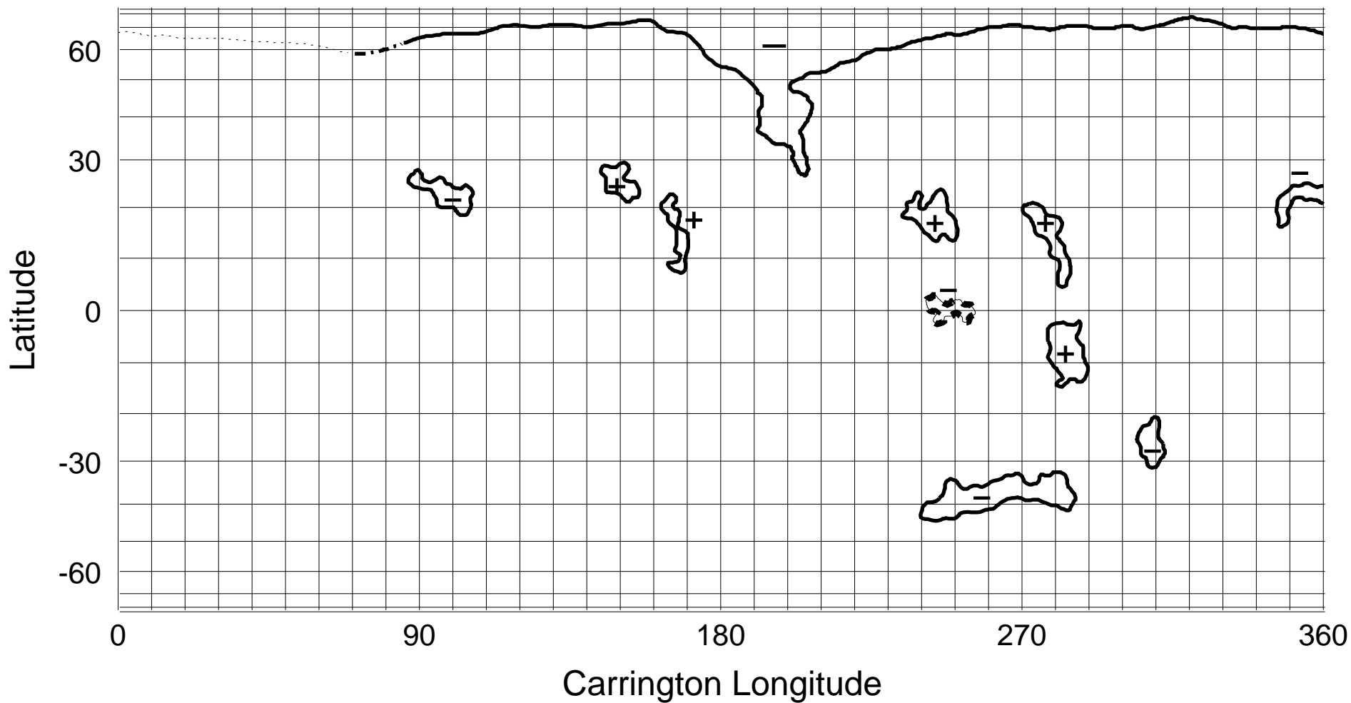
NSO/KP He I 1083 nm Coronal Hole Map: Carrington Rotation 1981
