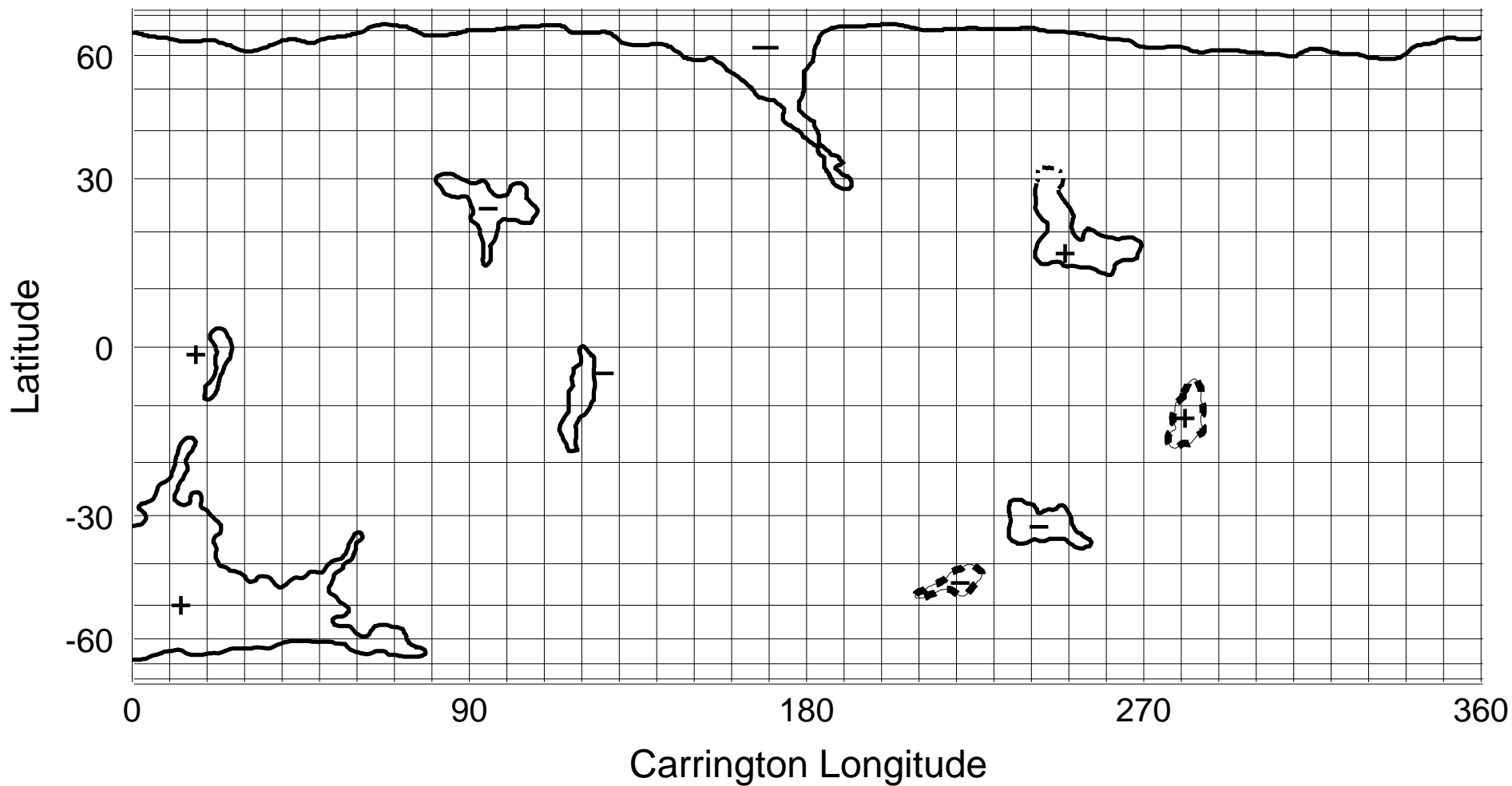
NSO/KP He I 1083 nm Coronal Hole Map: Carrington Rotation 1982
