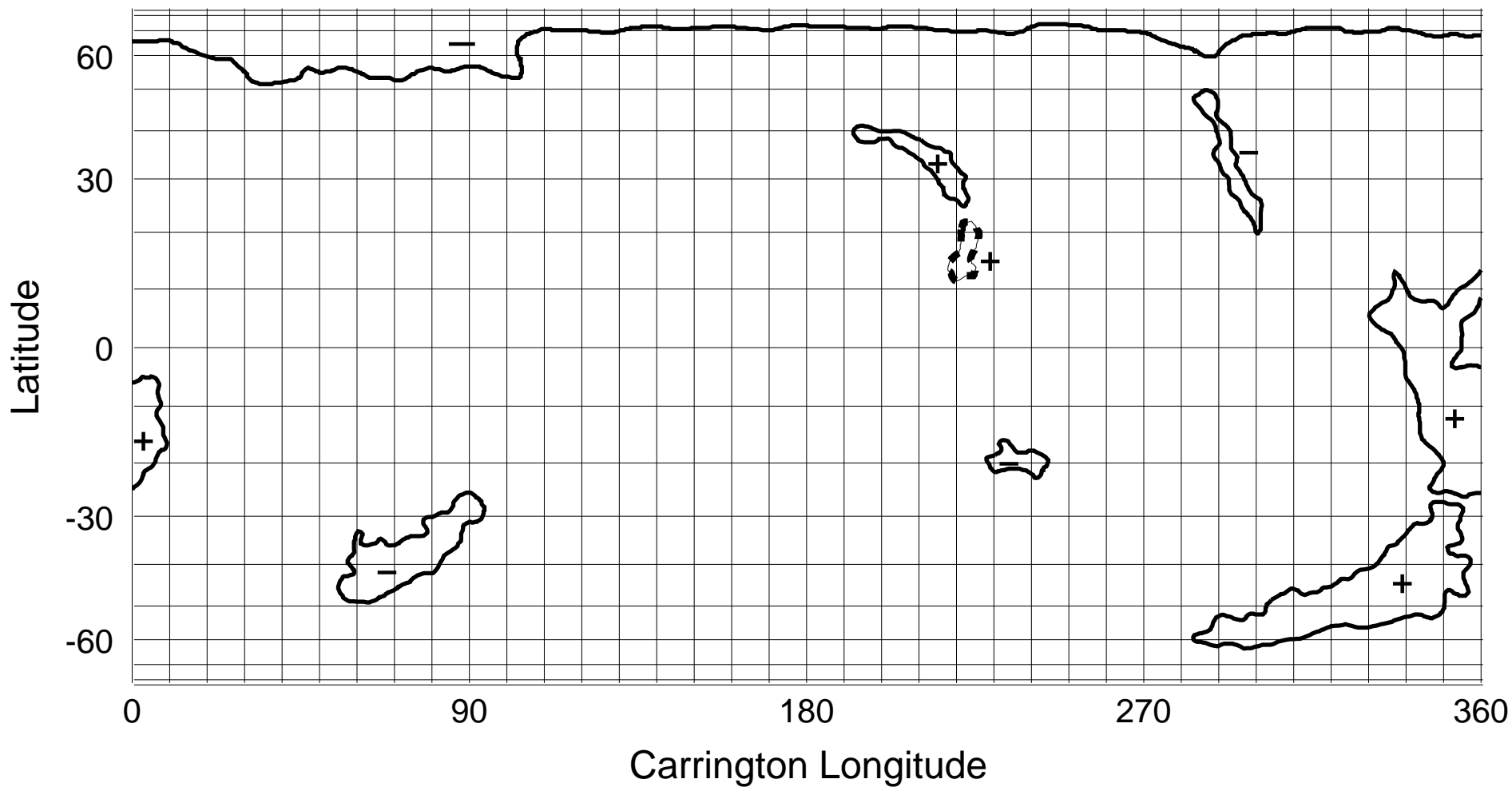
NSO/KP He I 1083 nm Coronal Hole Map: Carrington Rotation 1985
