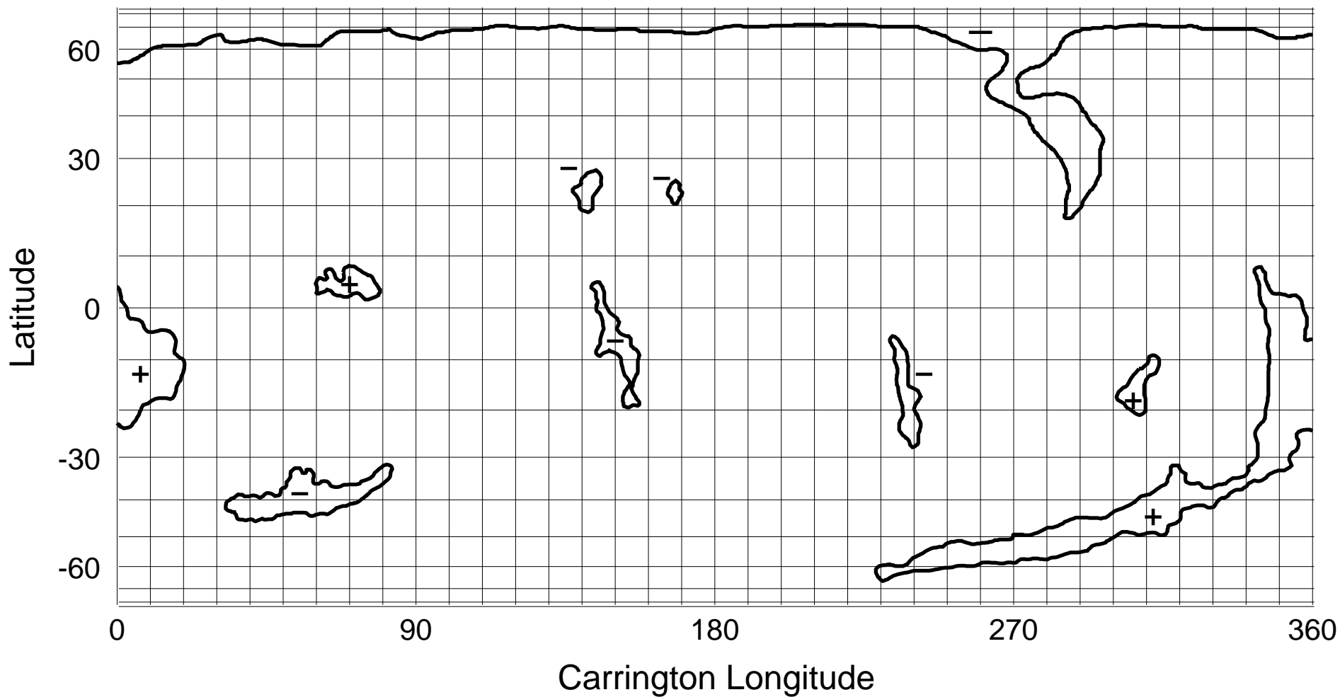
NSO/KP He I 1083 nm Coronal Hole Map: Carrington Rotation 1986
