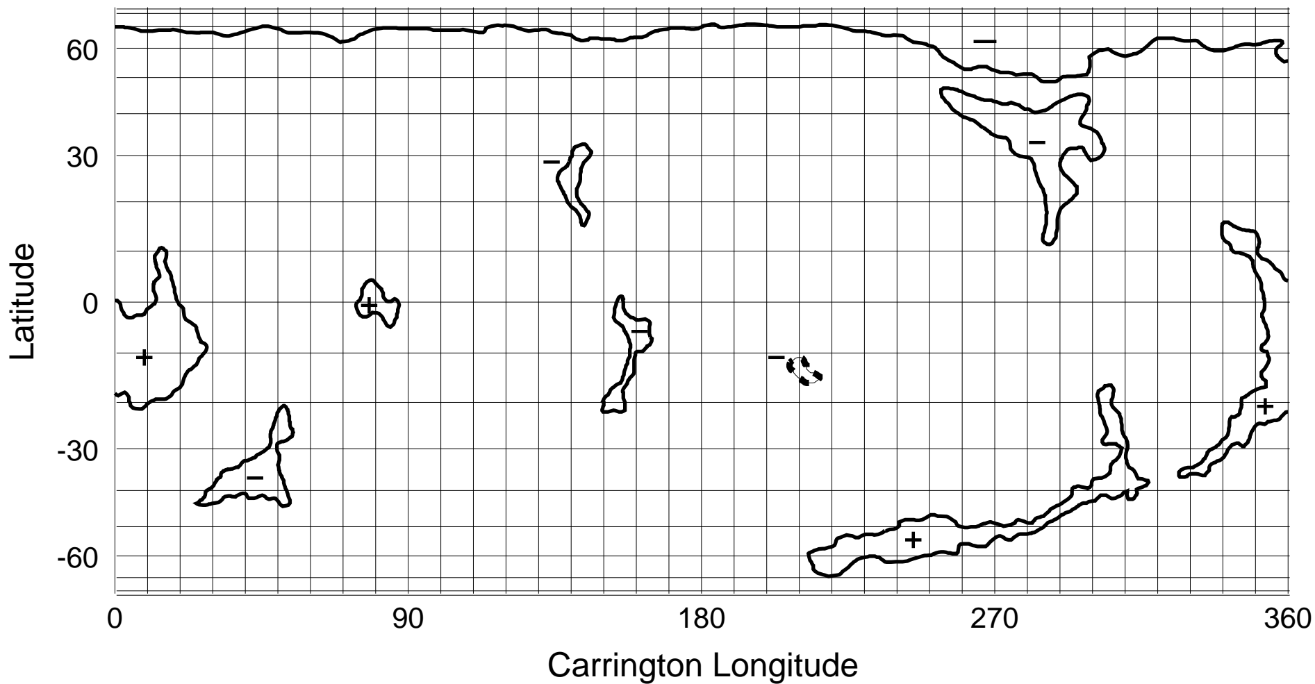
NSO/KP He I 1083 nm Coronal Hole Map: Carrington Rotation 1987
